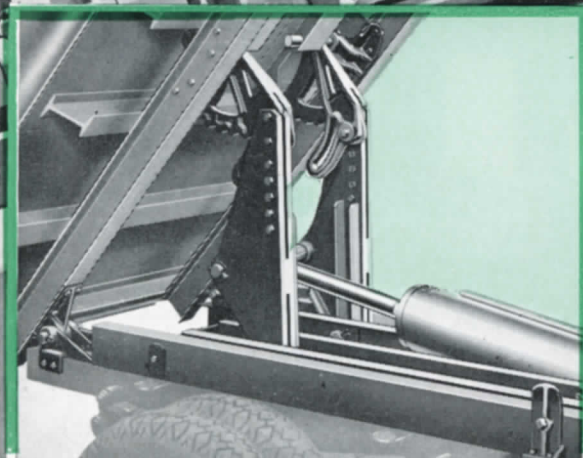
GALION GH-576 Hoist for 1 1-2 ton and 2 ton long wheelbase Dodge Trucks
