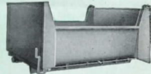
Model 8 —Straight side coal body. 75 to 128 cubic feet capacities. High head and endgate permit use of side boards to add 45 cubic feet capacity.
