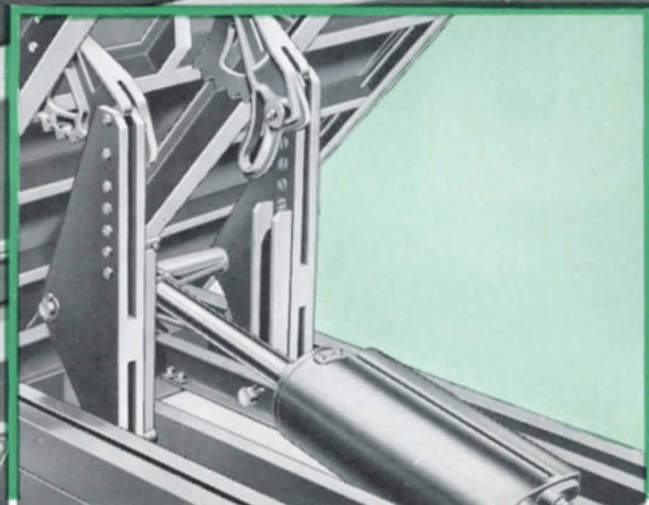
GALION GH-58 Hoist for heavy duty Dodge Trucks 3
