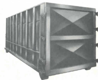
Open and Closed Roll-Off containers from fifteen to forty five cubic yards.
