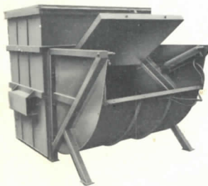
The Mini-Brute — Consists of a 1.5 cubic yard compactor coupled to a 6 cubic yard front or rear load container.
