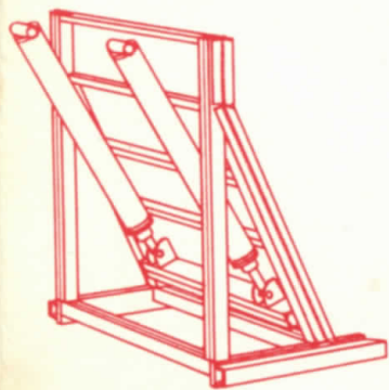
PUSH TYPE PACKING BLADE
