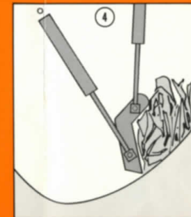
SWEEP: sweeps, and rolls material against rear hopper wall.
