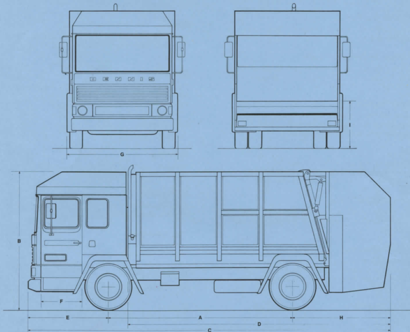
CHASSIS AND BODY DIMENSIONS (in mm.)
