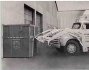
LoDal's exclusive triangle coupler connects the container in a matter of seconds. It couples at angles . . . and reaches out to pull containers into a full couple without moving the truck. This patented coupler is fast and efficient . . . a bonus in extra containers serviced per day.
