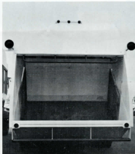
Rugged constructed Packing Panels with direct thrust. Results in greater compaction.
