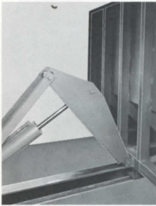
Scissor Mechanism In Retracted Position
