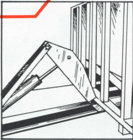
Scissor Mechanism In Retracted Position
